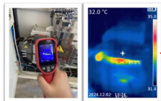
breaker inverter No.1 35.0 °C
